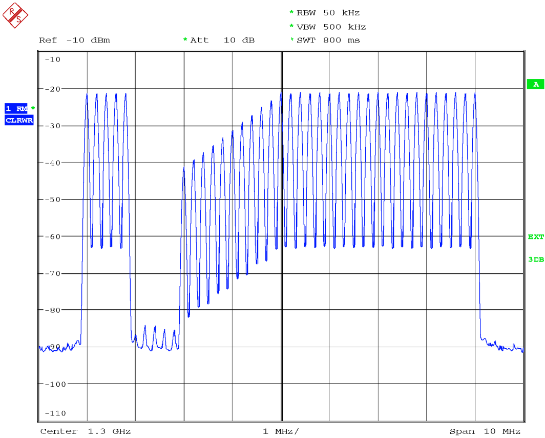
Example of multicarrier CW, with different carrier powers and some carriers switched off in the left half of the spectrum, I/Q level 0.5 V (meas.).
